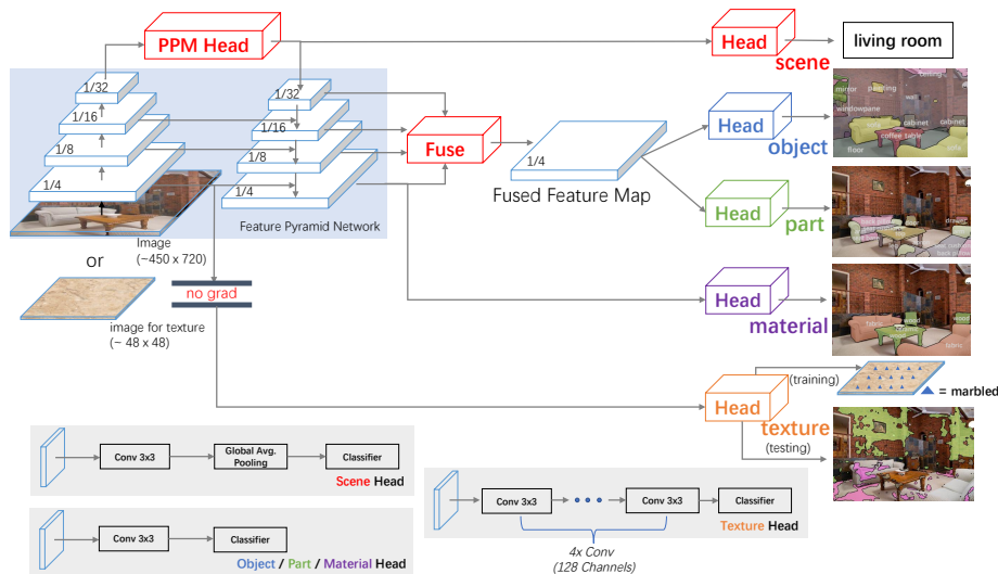
Fig. 4. UPerNet framework for Unified Perceptual Parsing. Top-left: The Feature Pyramid Network (FPN) [31] with a Pyramid Pooling Module (PPM) [16] appended on the last layer of the backbone network before feeding it into the top-down branch in FPN. Top-right: We use features at various semantic levels. Scene head is attached on the feature map directly after the PPM since image-level information is more suitable for scene classification. Object and part heads are attached on the feature map fused by all the layers put out by FPN. Material head is attached on the feature map in FPN with the highest resolution. Texture head is attached on the Res-2 block in ResNet [1], and fine-tuned after the whole network finishes training on other tasks. Bottom: The illustrations of different heads. Details can be found in Section 3.
