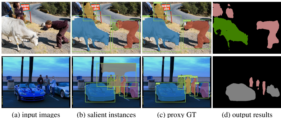
Fig. 1: Input images (a) are fed into a salient instance detection method (e.g., S^4 Net [16]) giving instances shown in colour in (b). Our system automatically generates proxy ground-truth data (c) by assigning correct tags to salient instances and rejecting noisy instances. Traditional fully supervised semantic/instance segmentation methods learn from these proxy ground-truth data; final generated segmentation results are shown in (d).
