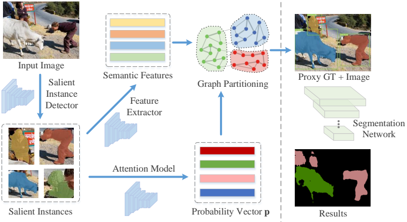
Fig. 2: Pipeline. Instances are extracted from the input images by a salient instance detector (e.g., S^4 Net [16]). An attention module predicts the probability of each salient instance belonging to a certain category using its intrinsic properties. Semantic features are obtained from the salient instances and used to build a similarity graph. Graph partitioning is used to determine the final tags of the salient instances. The fully supervised segmentation network (e.g., DeepLab [2] or Mask R-CNN [21]) is trained using the proxy ground-truth generated.
